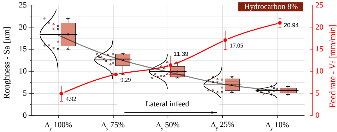
Figure 3: Technological performance behavior for dielectric fluid and \Delta y variation.
