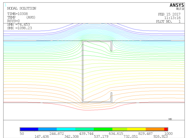
c) Temperature (critical time 171.8 min) - Case 1D
